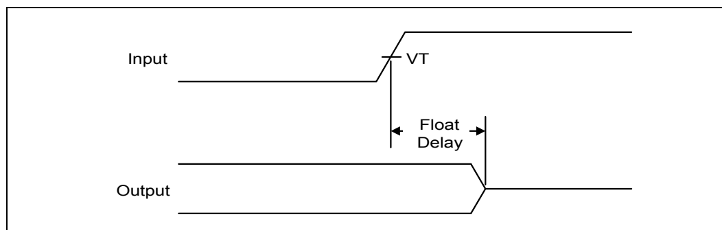
Figure 8-15. Float Delay
